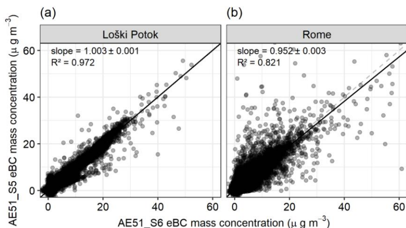
Fig. 1. Intercomparison for eBC mass concentrations (10-second median) measured by the AE51 S6 and AE51 S5 during the collocated MM in (a) Loški Potok, Slovenia and (b) Rome, Italy. Data were taken from two backpacks with identical instrumentation running simultaneously, side by side for each run, throughout the campaign. RMA regression was used to fit the two measurements. For IC details, see Tables 2, S1, S2, S3, and S4.
